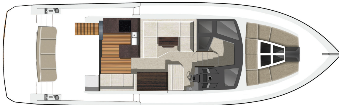
COCKPIT/MAIN DECK NOTE: Cockpit seating is different than shown for USA version. Galley to have cabinetry to starboard.
