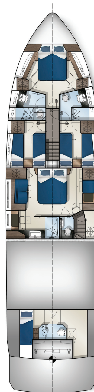
LOWER DECK
