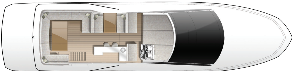
FLYBRIDGE DECK
