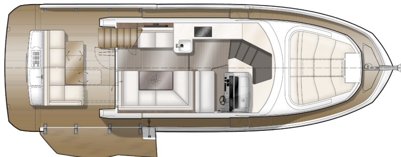
COCKPIT/MAIN DECK
